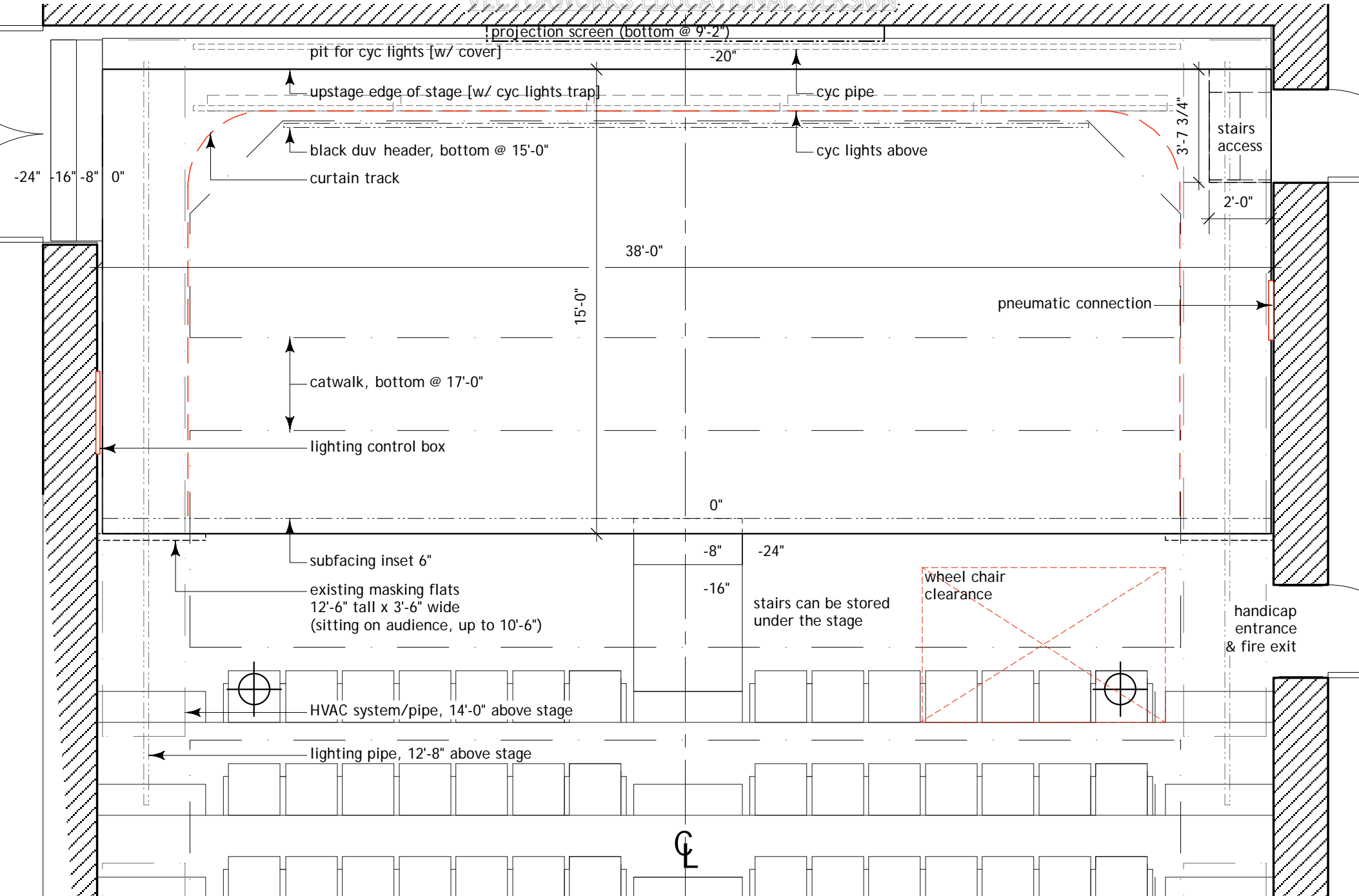
0' 2' 4' 6' 10' Theatre B at University of Iowa, 1/4" = 1'-0"
